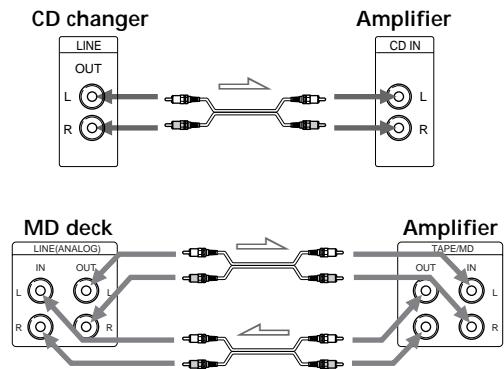
➡: Signal flow
