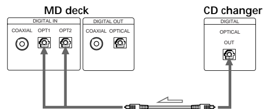
You can connect the optical cable to either OPT1 or OPT2
