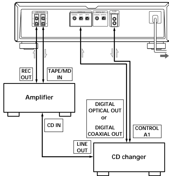
➡: Signal flow
