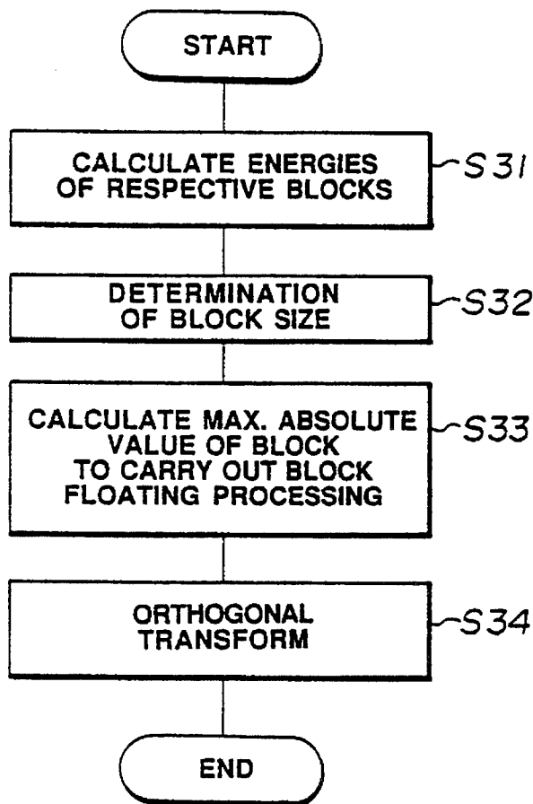
PRIOR ART FIG.16
